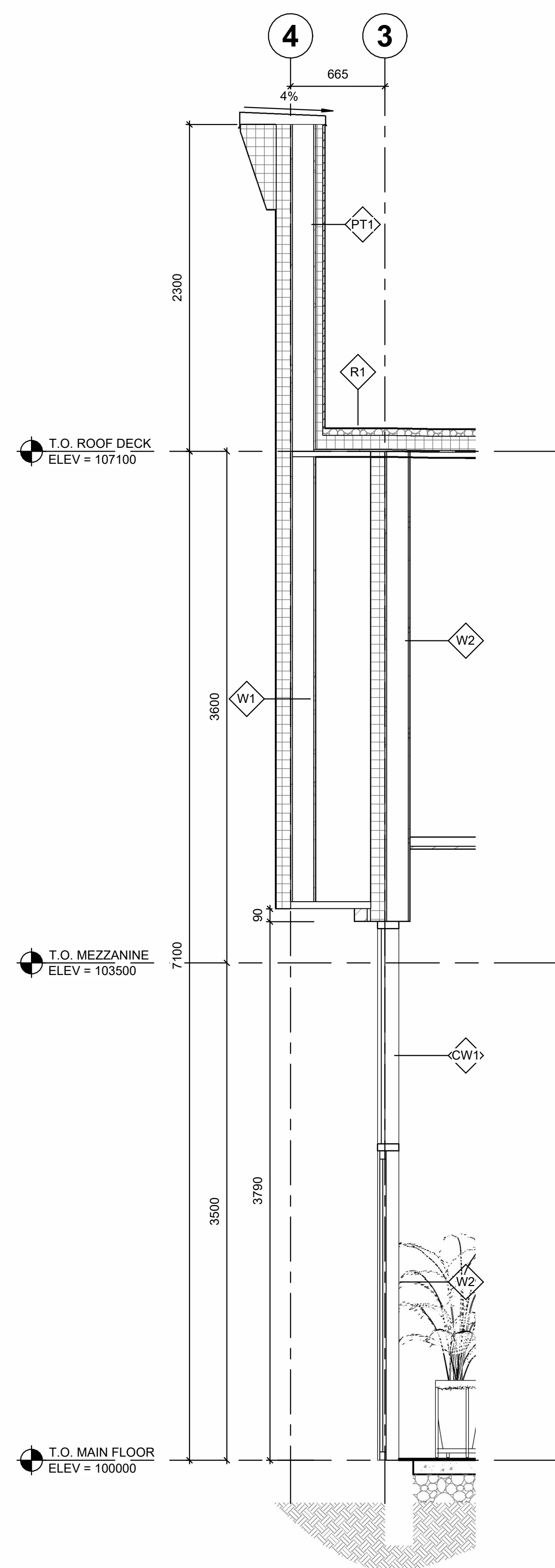
2 WALL SECTION A4.1 SCALE = 1 : 25
