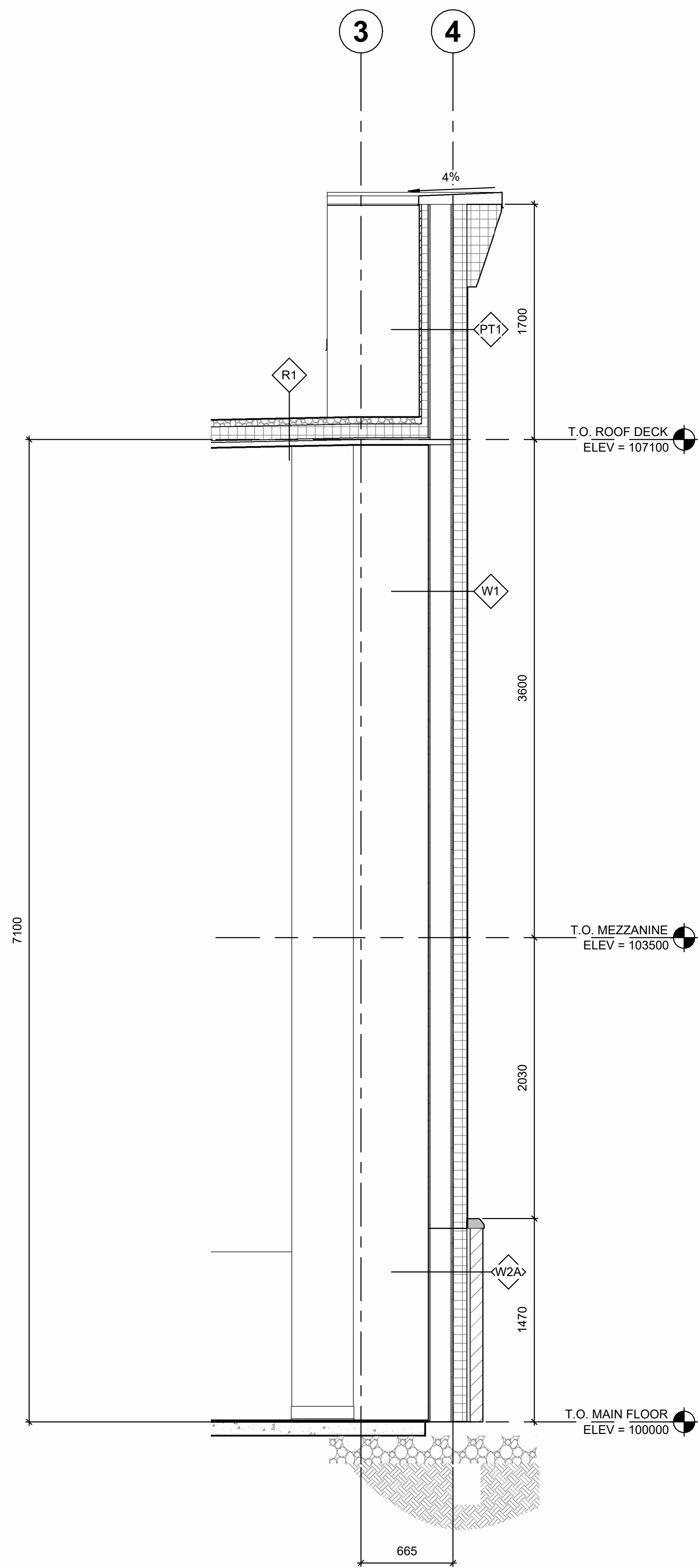
1 WALL SECTION
