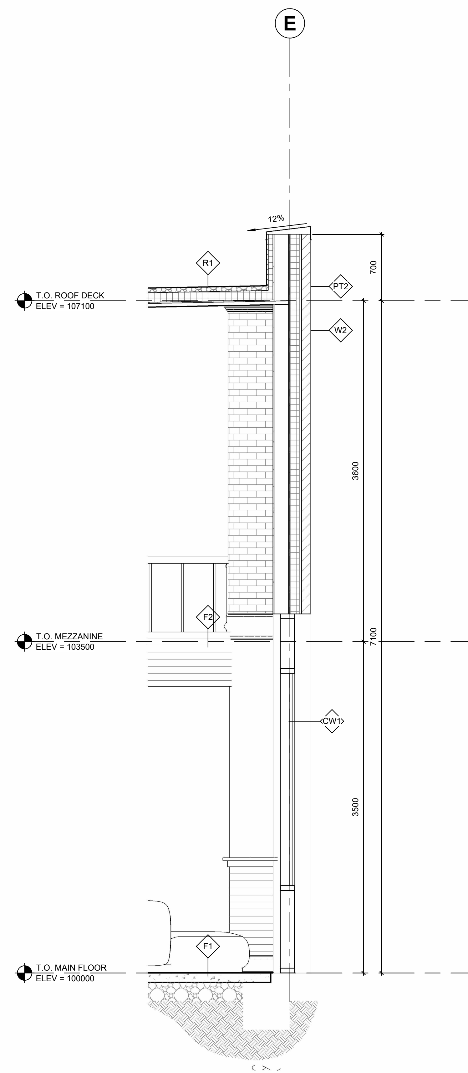
3 WALL SECTION
